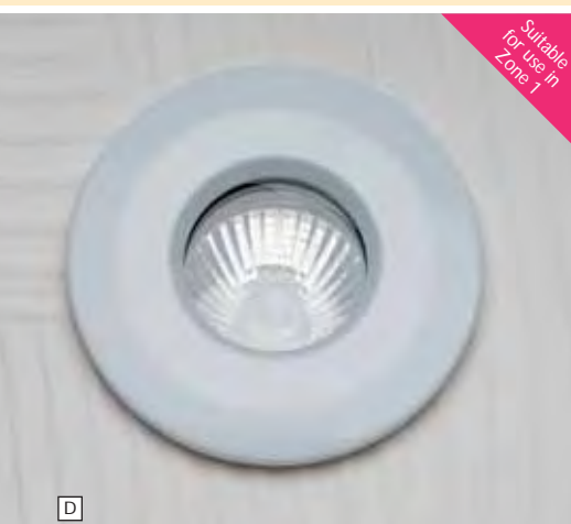
D GU10 Mains Voltage IP65 Shower Downlight Cut-out: 72mm. Void depth: 118mm. Rim Dia: 87mm. Lamp: 35W GU10 aluminium reflector. Quote: MM72020 (White finish) Quote: MM72021 (Polished Chrome finish) Quote: MM72022 (Brushed Chrome finish)
